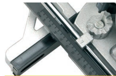
METAL PARALLEL GUIDE FENCE WITH DISTANCE SCALE (POWX093)
